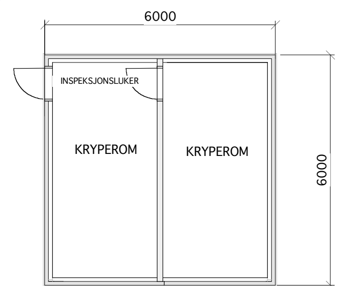
PLAN FUNDAMENT
